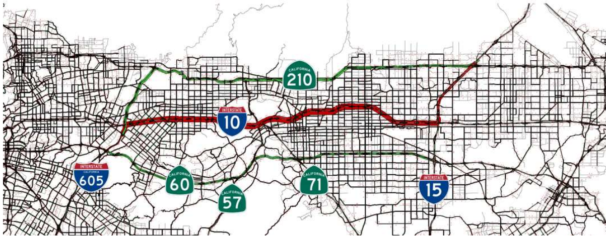
Daily Truck Volume Differences: Alt. 3 – Alt. 1 (Red = Increase Green = Decrease)
